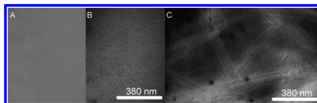
Figure 4. Transmission electron microscopy images of compound 2 at a concentration of 50 \mu M [(A) blank; (B) pH 5.5; (C) pH 7.5].
